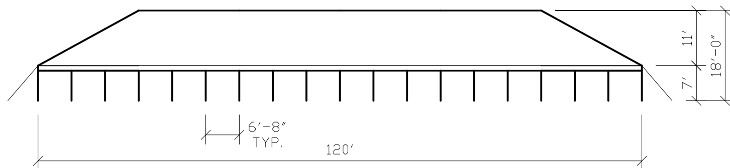
SIDE ELEVATION
